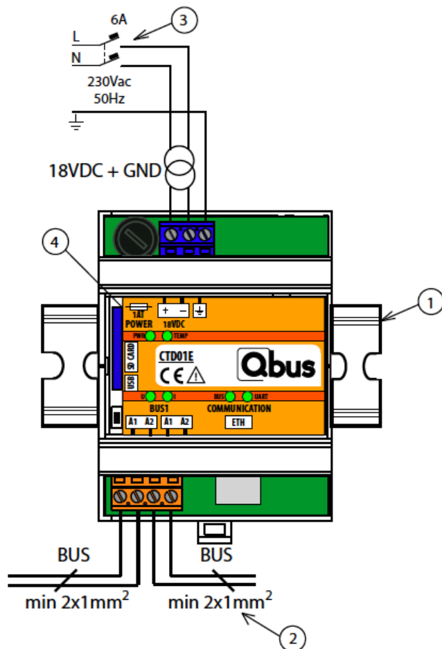
Figure 2 : Connection controller CTD01E
